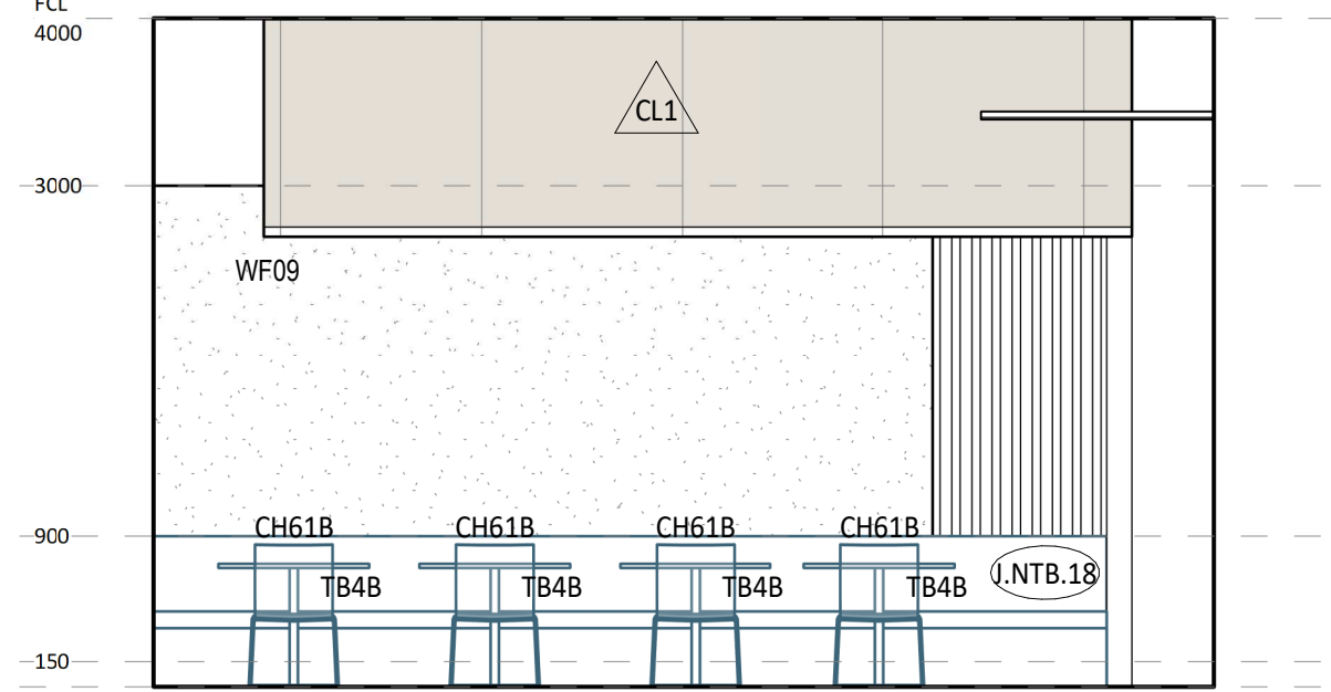
5 ELEVATION DETAIL 60-044 1:50
